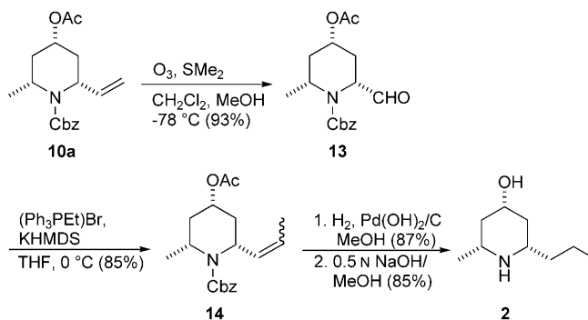
Scheme 6. Synthesis of the spruce alkaloid 2 .
