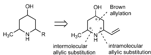
Scheme 2. Retrosynthetic analysis of 2,6-disubstituted hydroxypiperidines.
