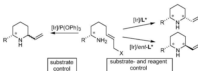
Scheme 1. Double stereodifferentiation: interplay between substrate- and reagent-induced selectivity ([Ir] = Ir catalyst; L* = L1 or L2).
