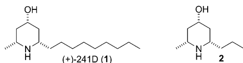
Figure 1. Examples of naturally occurring 2,6-disubstituted 4-hydroxypiperidines.
