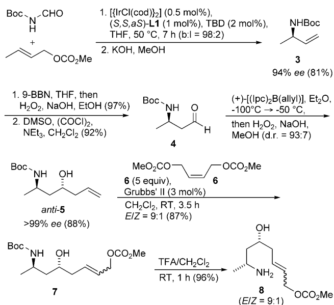
Scheme 3. Synthesis of the cyclization precursor 8 .
