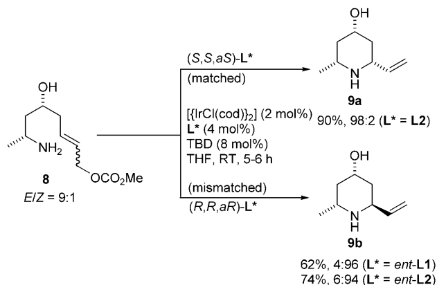
Scheme 4. Ir-catalyzed cyclizations.
