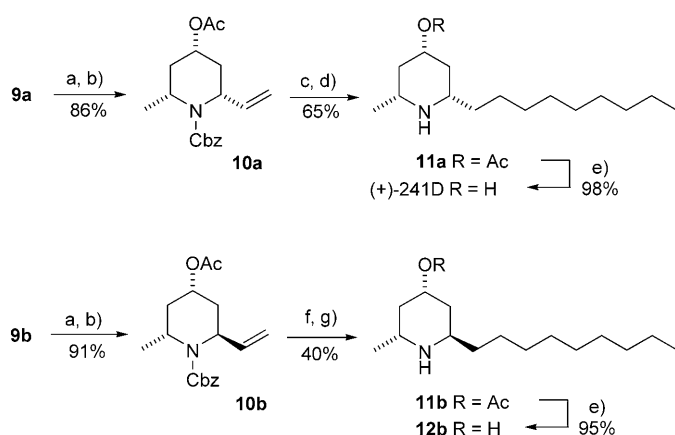
Scheme 5. Synthesis of (+)-241 D ( 1 ) and its C6-epimer 12b : a) CbzCl, Na 2 CO 3 , CH 2 Cl 2 /H 2 O, 0 °C → RT; b) Ac 2 O, pyridine; c) 1-Nonene (10 equiv), Grubbs' II catalyst (10 mol %), CH 2 Cl 2 , 5 h, reflux (71 %, 91 % corr.); d) H 2 , Rh/C (5 mol %), MeOH, 1 h, RT (92 %); e) 0.5 N NaOH/MeOH; f) 1-Nonene (10 equiv), Grubbs' II catalyst (10 mol %), CH 2 Cl 2 , 8 h, reflux (46 %, 99 % corr.); g) H 2 , Pd(OH) 2 /C (5 mol %), MeOH, 1 h, RT (86 %).
