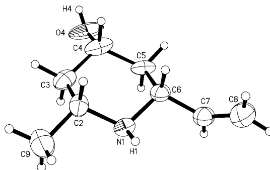
Figure 2. Molecular structure of 9a from single-crystal X-ray structure analysis.
